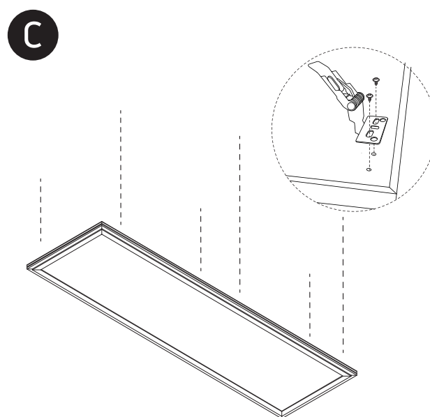
Recessed mount applications using optional kit 050108 (2 Sets).
