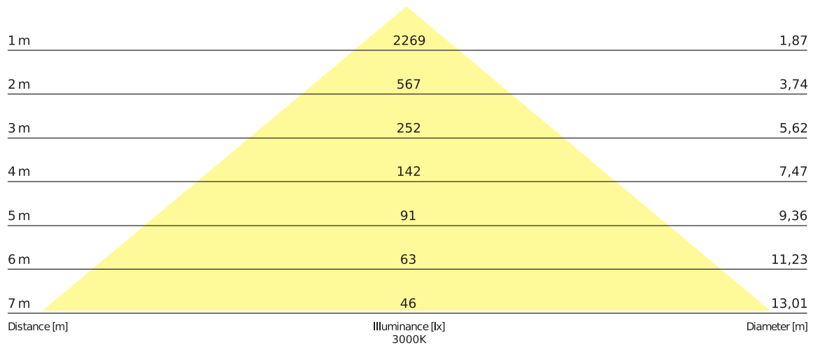
Beam cone diagram Beam angle 86°
