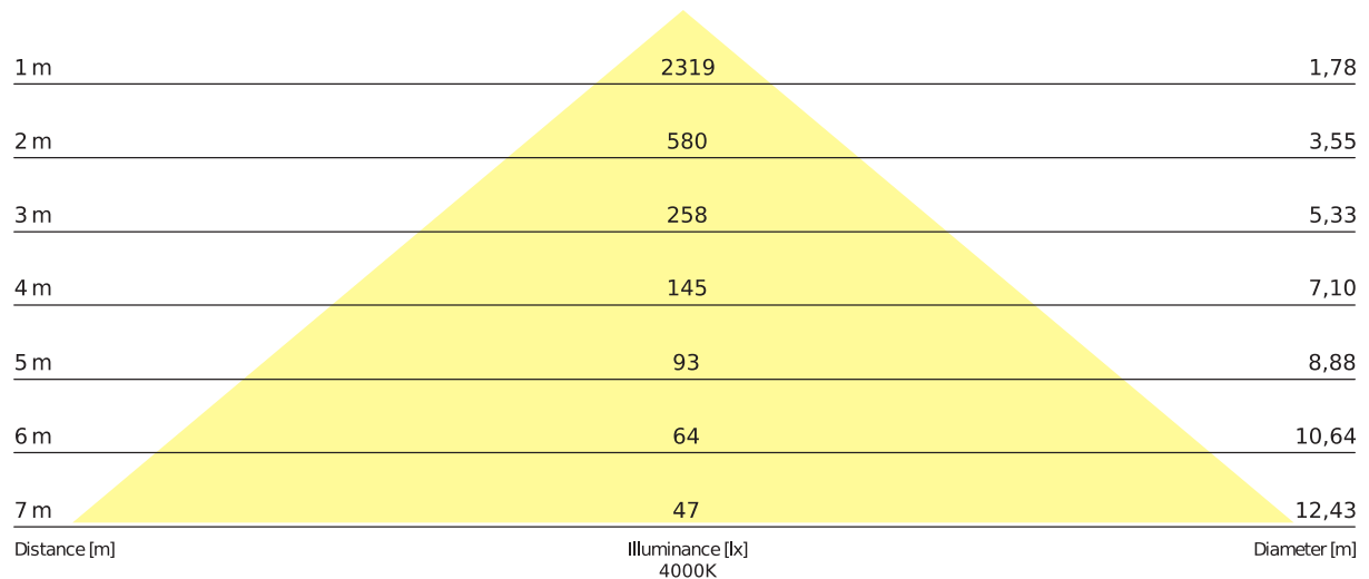
Beam cone diagram Beam angle 83°
