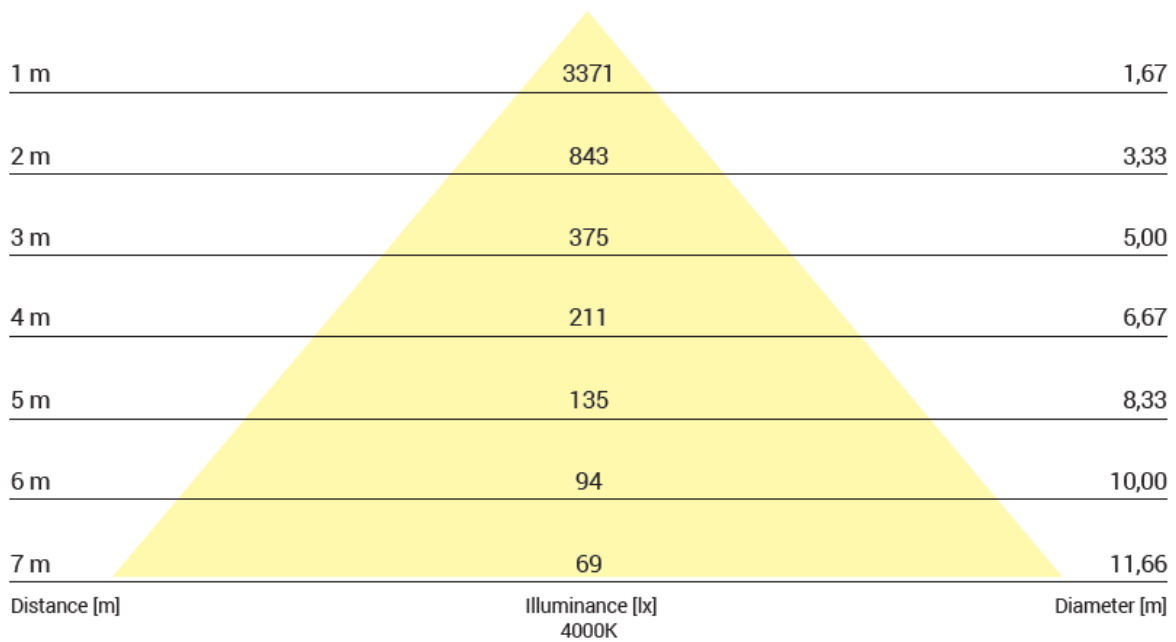
Beam cone diagram Beam angle 80°
