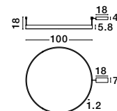
MOTIF . 9063607 Dimmable Sandy Black Aluminium & Acrylic LED 60 Watt 230 Volt 4551.55lm 3000K IP20 D: 100 W: 1.2 H: 18 cm
