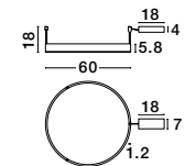
MOTIF . 9063601 Dimmable Sandy Black Aluminium & Acrylic LED 45 Watt 230 Volt 3350.75lm 3000K IP20 D: 60 W: 1.2 H: 18 cm
