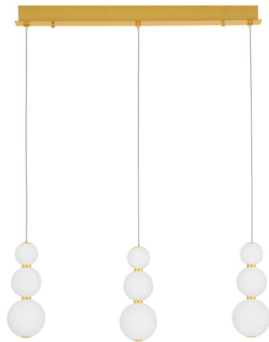
FLEA - 9695243 Dimmable Gold Metal Opal Glass LED 24 Watt 230 Volt 2264.76 Lm 3000K IP20 L: 70 H: 150 cm LED WARM WHITE DRIVER INCL.
