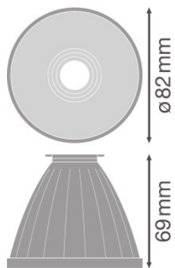
TRACK SP REFLECTOR D95 SP
