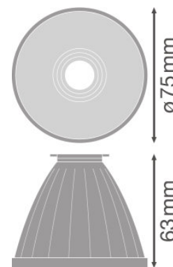
TRACK SP REFLECTOR D85 SP
