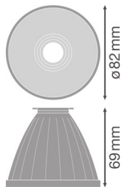
TRACK SP REFLECTOR D95 FL
