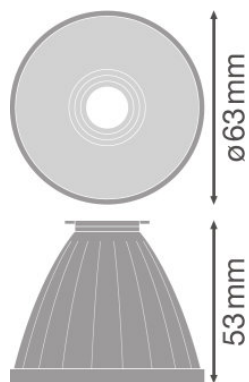
TRACK SP REFLECTOR D75 SP
