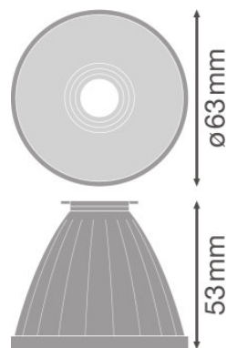
TRACK SP REFLECTOR D75 FL
