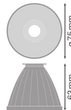
TRACK SP REFLECTOR D85 FL
