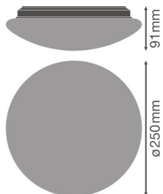
SF CIRCULAR 250 S 13 W 3000 K IP44 WT, SF CIRCULAR 250 S 13 W 4000 K IP44 WT
