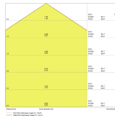
SF BLKH 250 S 10W/4000K WT IP65
