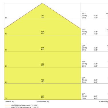
SF BLKH 250 S 10W/3000K WT IP65
