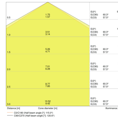
O FACADE SPOT 8 W 3000 K IP54 WT
