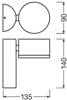
O FACADE SPOT 8 W 3000 K IP54 GY, O FACADE SPOT 8 W 3000 K IP54 WT
