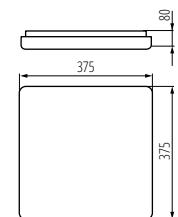
QADI LED 32W
