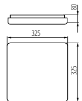
QADI LED 18W, QADI LED 24W
