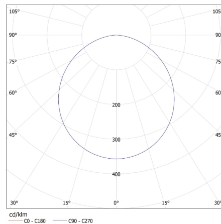
MILEDO (кат 31077) SP LED N 6W NW-R / LDC (Polar)
