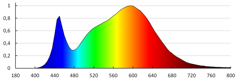
MILEDO (кат 31077) SP LED N 6W NW-R / LDC (Polar)
