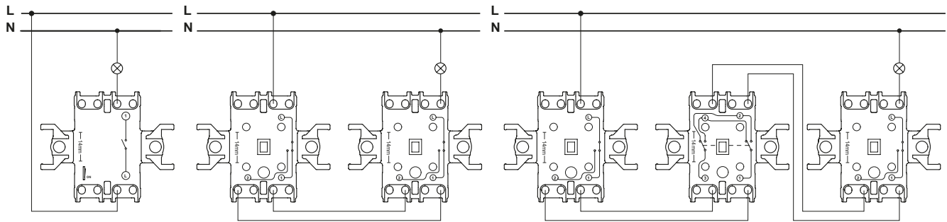
1-way switch
